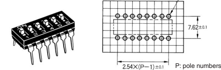
PCB Dimensions (Top View)
