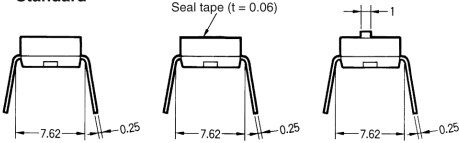
Flat Actuator Standard
