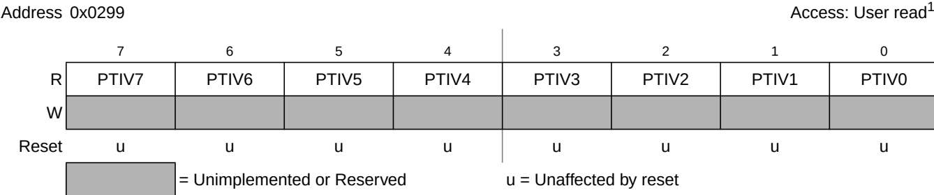
Figure 2-80. Port V Input Register (PTIV)
