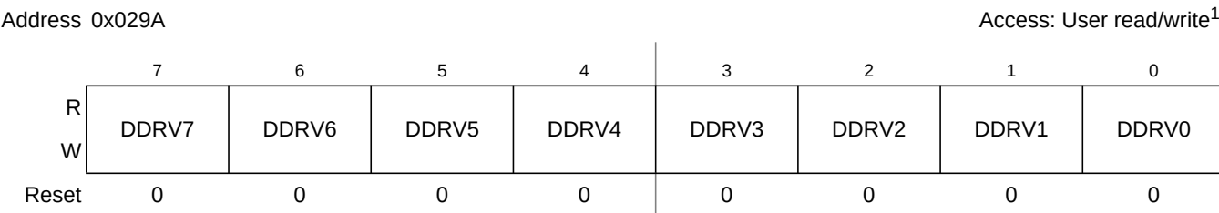
Figure 2-81. Port V Data Direction Register (DDRV)
