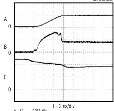
TURN-ON WAVEFORMS R_L = 60\Omega , C_L = 100\mu F
