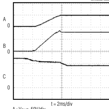
TURN-ON WAVEFORMS R_L = 60\Omega , C_L = 10\mu F
