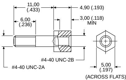
Jackpost
