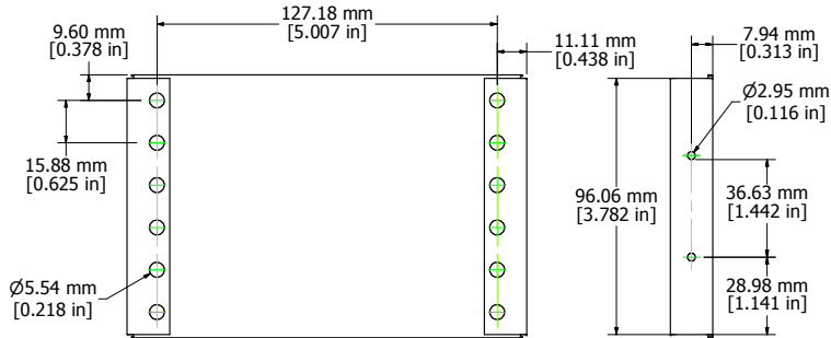
END PLATES
