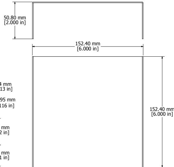
BOTTOM/TOP ENCLOSURE
