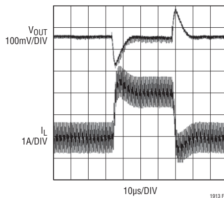
Figure 3. Transient Load Response of the LT1913 Front Page Application as the Load Current is Stepped from 1A to 3A. V_{OUT} = 5V
