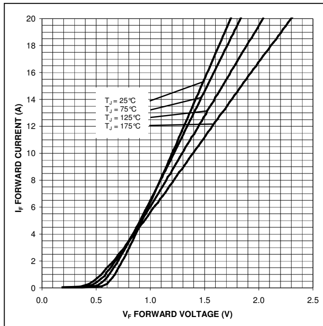
Figure 1. Forward Characteristics
