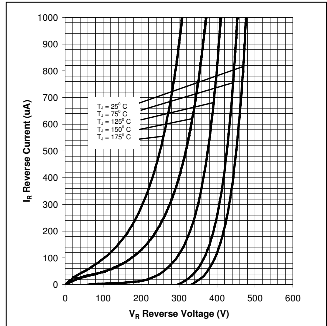
Figure 2. Reverse Characteristics
