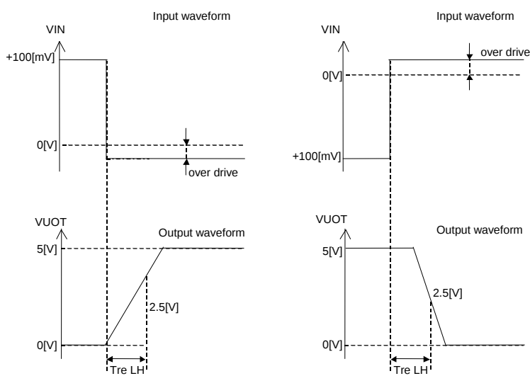
Fig.90 Response Time
