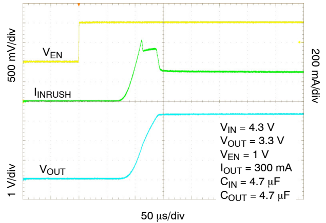
Figure 23. Enable Turn-on Response – C_{OUT} = 4.7 \mu\text{F} , I_{OUT} = 300 \text{ mA}
