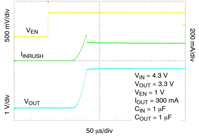
Figure 21. Enable Turn-on Response – C_{OUT} = 1 \mu\text{F} , I_{OUT} = 300 \text{ mA}
