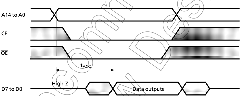
Timing Waveforms of Read Operation
