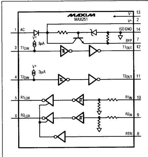
Figure 2. MAX251 Block Diagram
