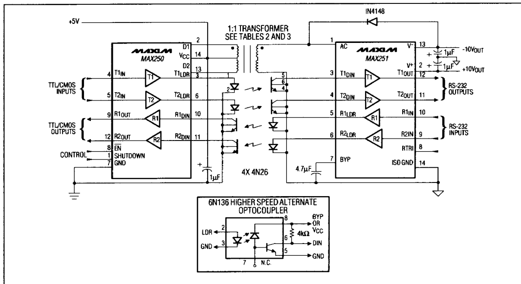
Figure 3. Isolated RS-232 Interface
