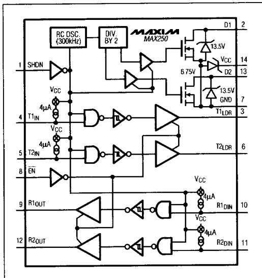
Figure 1. MAX250 Block Diagram
