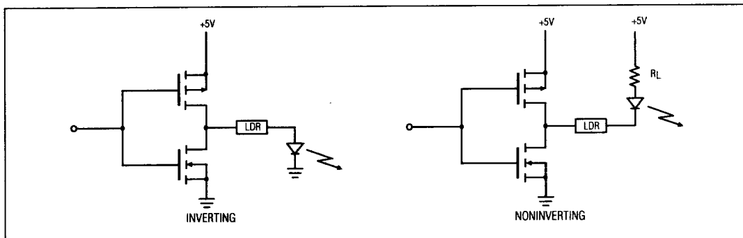
Figure 5. LDR Output Structure
