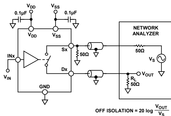
Figure 27. Off Isolation
