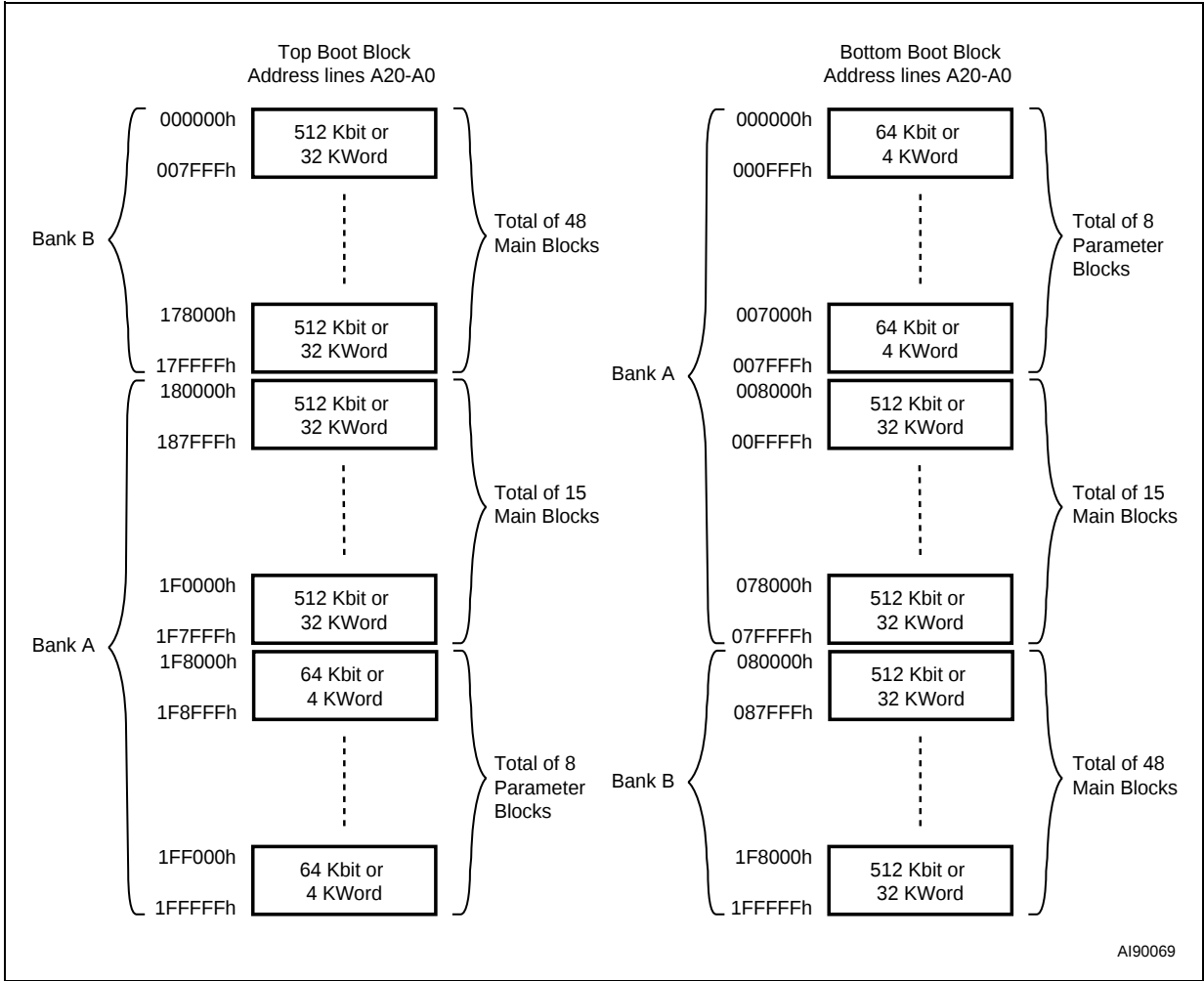
Figure 3. Memory Map
