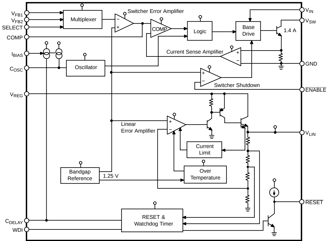
Figure 1. Block Diagram
