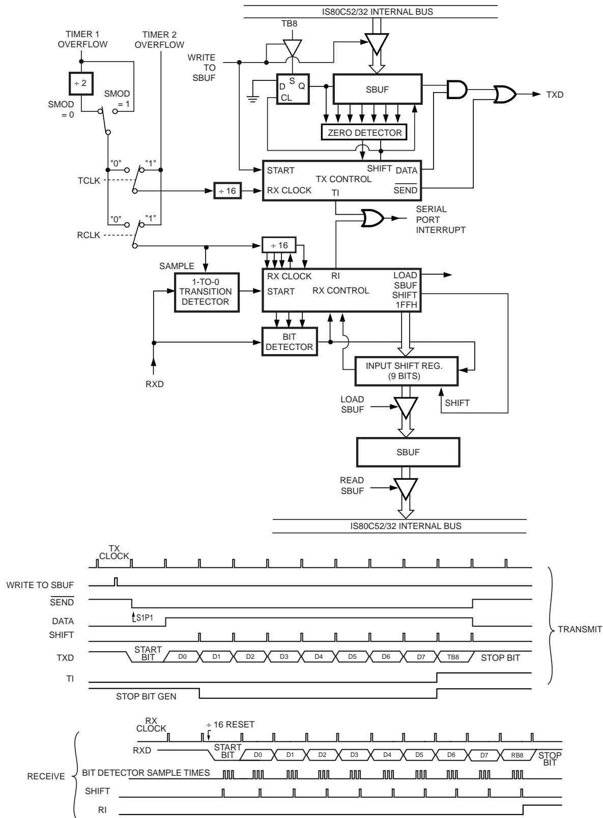
Figure 18. Serial Port Mode 3
