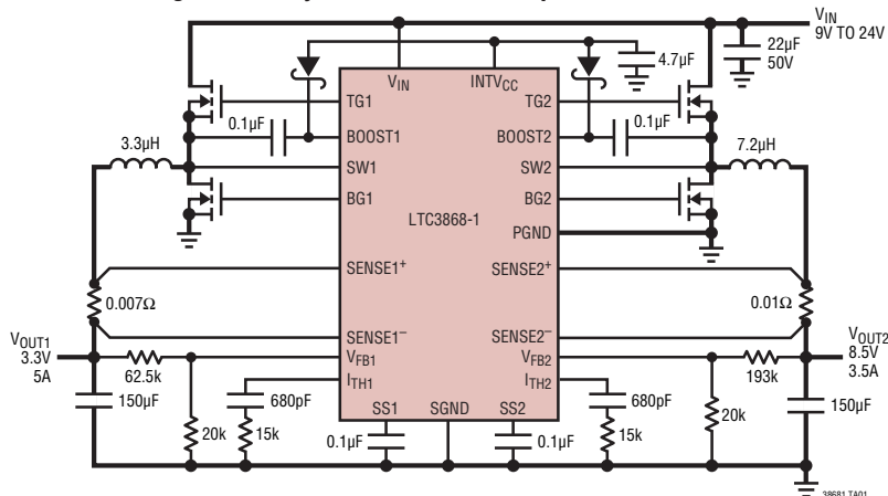
High Efficiency Dual 8.5V/3.3V Step-Down Converter
