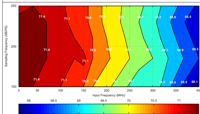
Figure 35. Signal-to-Noise Ratio (0-dB Gain)
