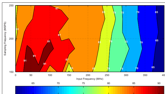
Figure 33. Spurious-Free Dynamic Range (0-dB Gain)
