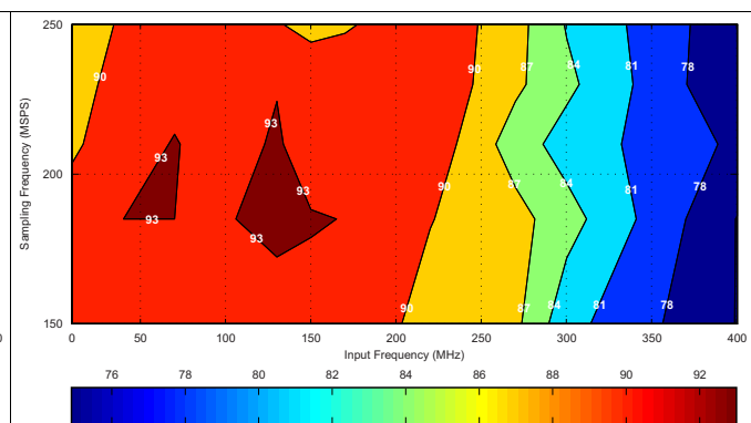
Figure 34. Spurious-Free Dynamic Range (6-dB Gain)
