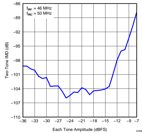
Figure 8. Two-Tone IMD3 vs Input Amplitude
