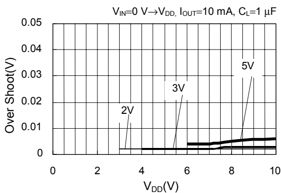
V_{DD} dependencies of overshoot at powering on
