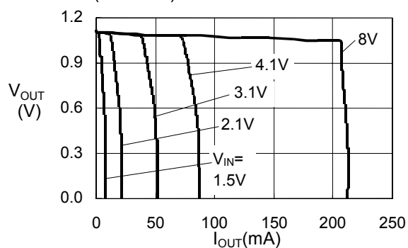
S-817B11A(Ta=25°C)
