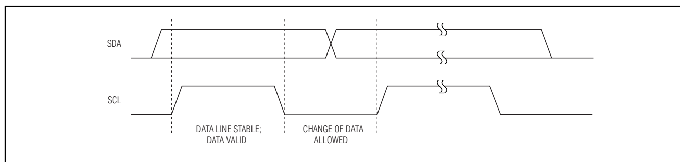
Figure 4. Bit Transfer
