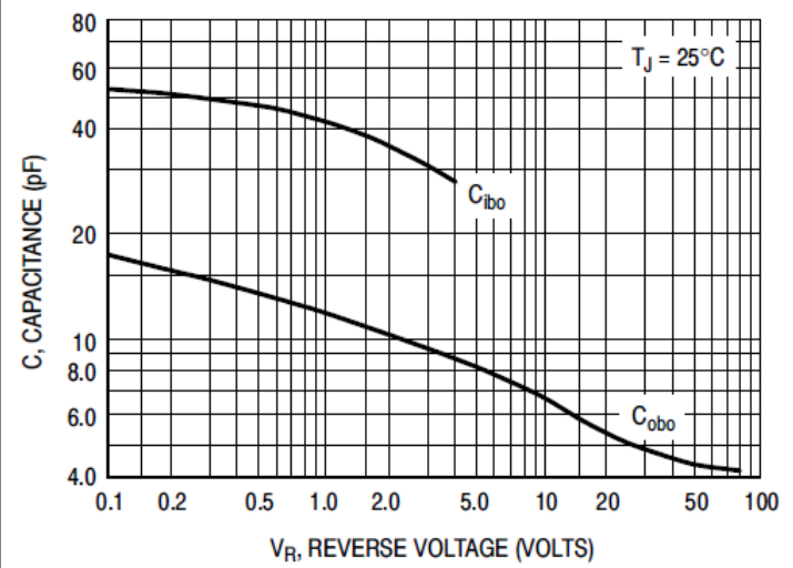
Fig.2 Capacitance
