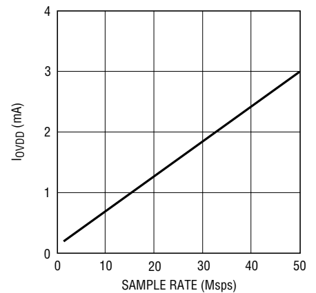
LTC2237: I_{OVD} vs Sample Rate, 5MHz Sine Wave Input, -1dB, O_{VDD} = 1.8\text{V}
