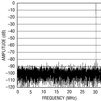
LTC2238: 8192 Point FFT, f_{IN} = 30\text{MHz} , -1dB, 2V Range, 65Mps
