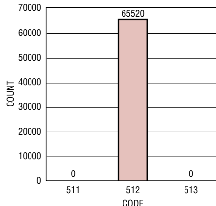
LTC2238: Grounded Input Histogram, 65Mps
