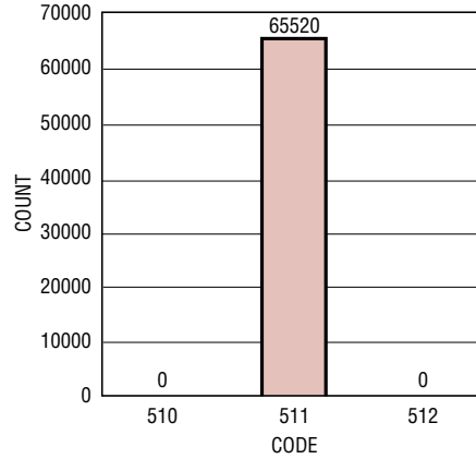
LTC2237: Grounded Input Histogram, 40\text{Mpsps}
