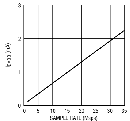
LTC2236: I_{OVPD} vs Sample Rate, 5\text{MHz} Sine Wave Input, -1\text{dB} , O_{VDD} = 1.8\text{V}
