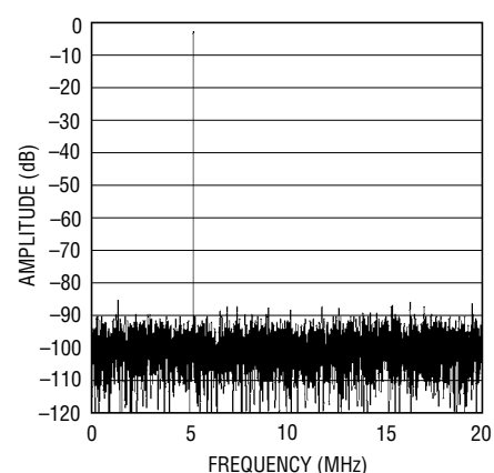
LTC2237: 8192 Point FFT, f_{IN} = 5\text{MHz} , -1dB, 2V Range, 40Msps
