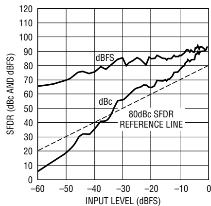
LTC2236: SFDR vs Input Level, f_{IN} = 5\text{MHz} , 2\text{V} Range, 25\text{Mpsps}
