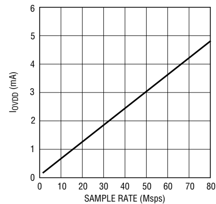
LTC2238: I_{VDD} vs Sample Rate, 5MHz Sine Wave Input, -1dB, V_{DD} = 1.8\text{V}
