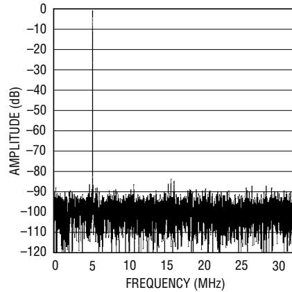
LTC2238: 8192 Point FFT, f_{IN} = 70\text{MHz} , -1dB, 2V Range, 65Mps
