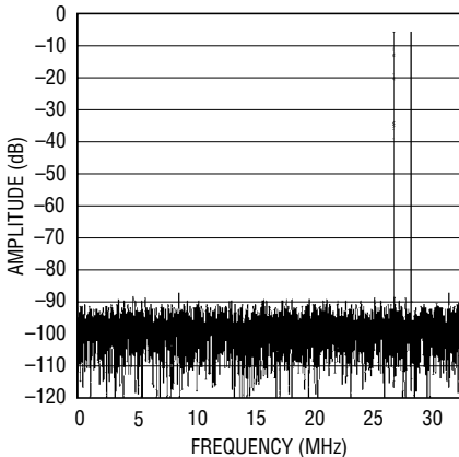
LTC2238: 8192 Point 2-Tone FFT, f_{IN} = 28.2\text{MHz} and 26.8\text{MHz} , -1dB, 2V Range, 65Mps
