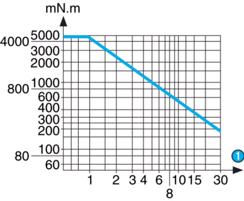
Torque/speed curves 80 527 0
