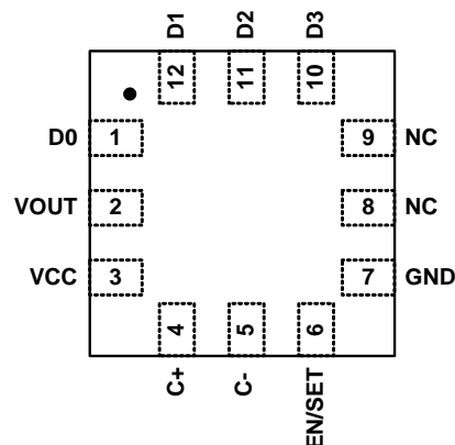
Figure 6.1 Pin Configuration ZLED7012 – Top View
