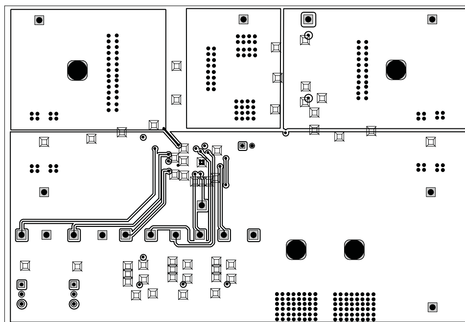
Figure 5. Layer 2
