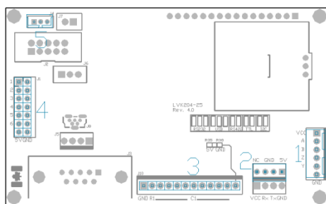
Figure 8: RS422 Connections
