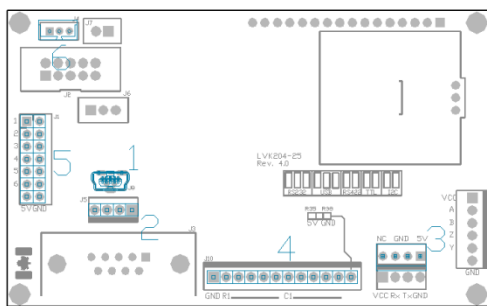
Figure 6: USB Connections
