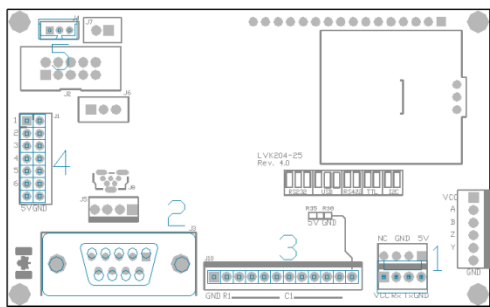
Figure 3: Standard Connections
