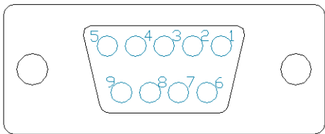
Figure 12: Serial DB9 Connector
