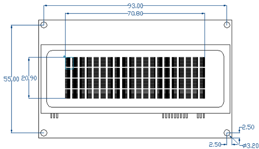
Figure 24: LVK204-25 Dimensional Drawing
