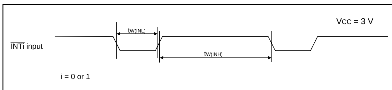
Figure 5.22 External Interrupt \overline{INTi} Input Timing Diagram when Vcc = 3 V
