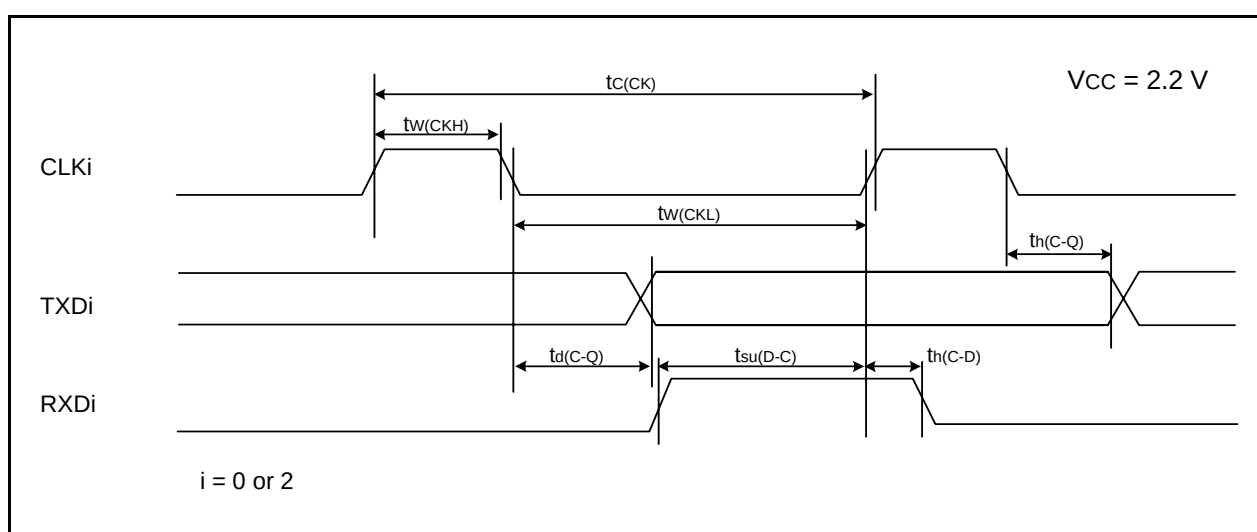
Figure 5.13 Serial Interface Timing Diagram when Vcc = 2.2 V
