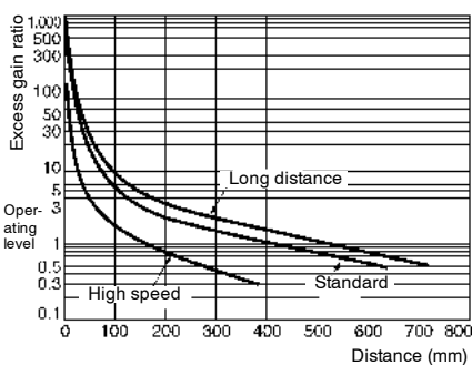
E32-DC200 with E3X-DAN amplifier (Reflective)
