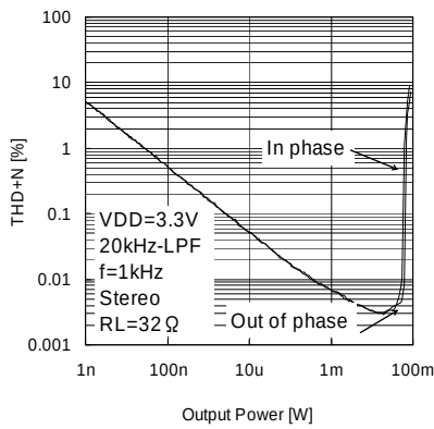
Fig. 37 THD+N vs. Output Power ( V_{DD}=3.3V , R_L=32\Omega )
