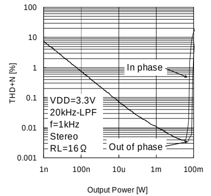
Fig.36 THD+N vs. Output Power ( V_{DD}=3.3V , R_L=16\Omega )
