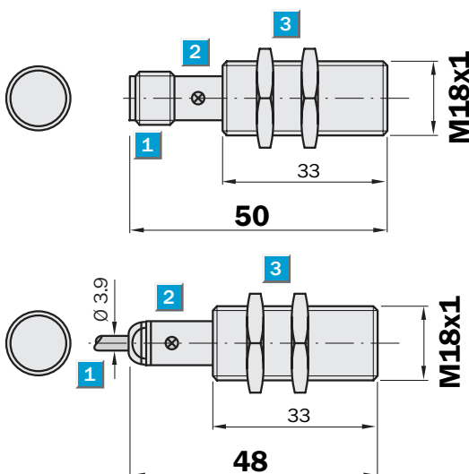
Dimensional drawing
