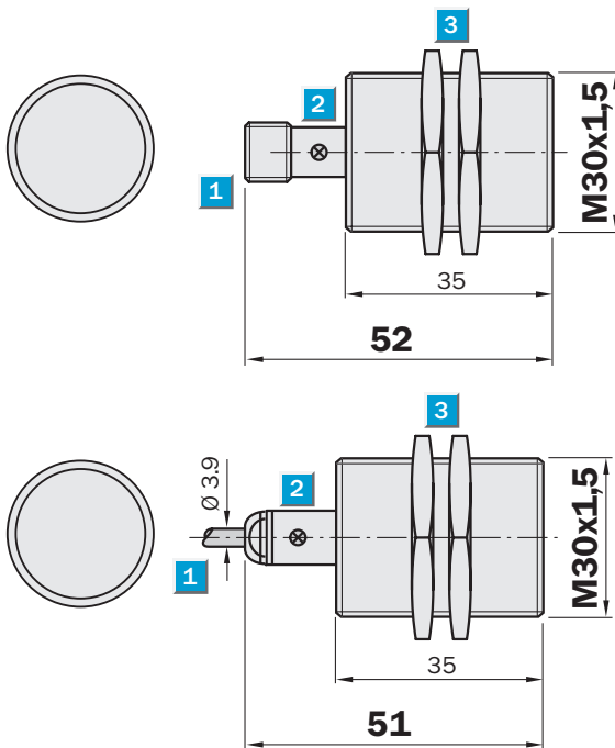
Dimensional drawing
