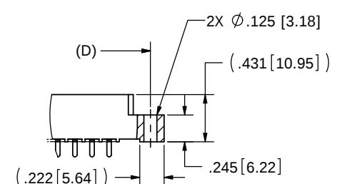
MOUNTING STYLE DR_D
