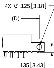
MOUNTING STYLE DR_S
