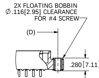
MOUNTING STYLE DR_F
