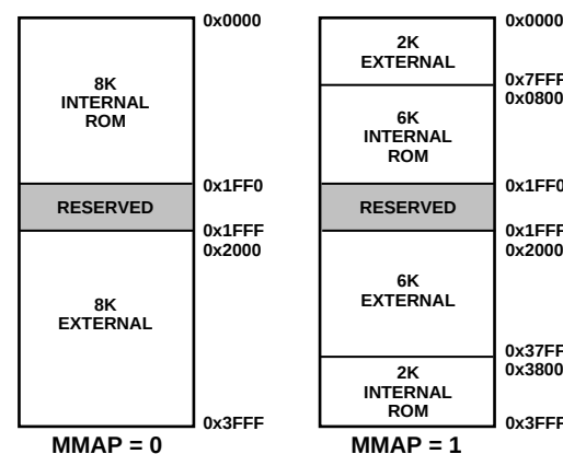
Figure 5. ADSP-2161/ADSP-2162 Program Memory Maps
