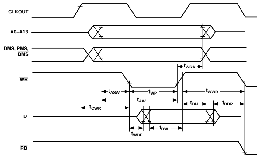
Figure 25. Memory Write
