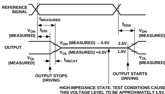
Figure 19. Output Enable/Disable
