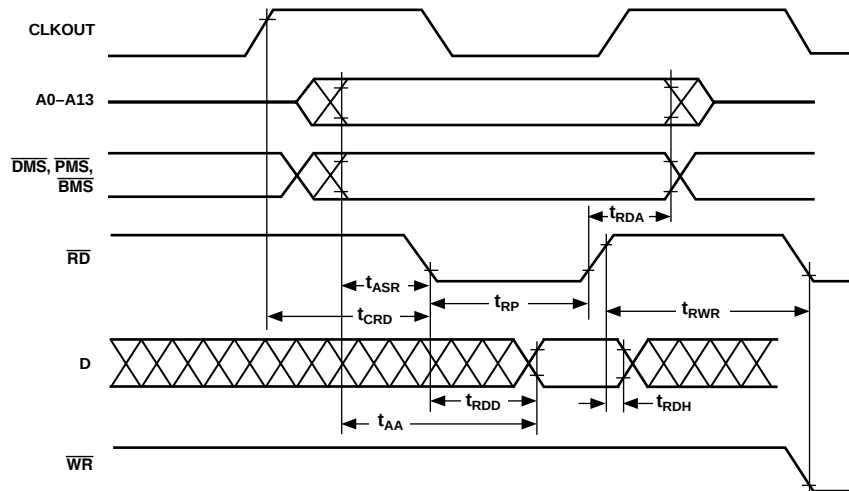
Figure 30. Memory Read
