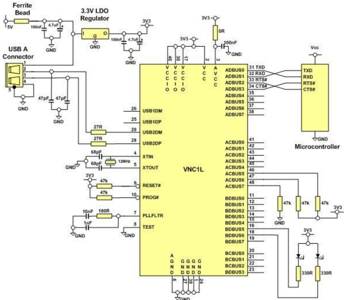
Figure 7.1 VNC1L Schematic (MCU - UART Interface)
