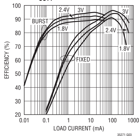
Efficiency vs Load Current and V_{IN} for V_{OUT1} = 3.3\text{V} at 1.2\text{MHz}
