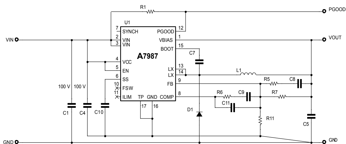
Figure 1. Application schematic
