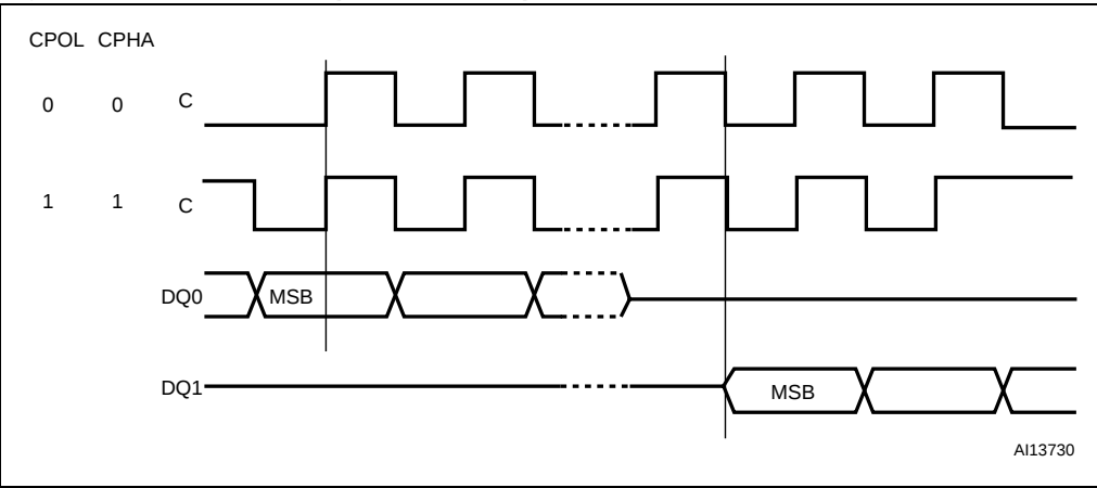
Figure 6. Extended SPI protocol example
