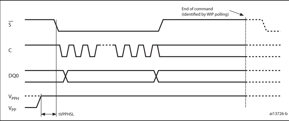
Figure 107. VPP_H timing
