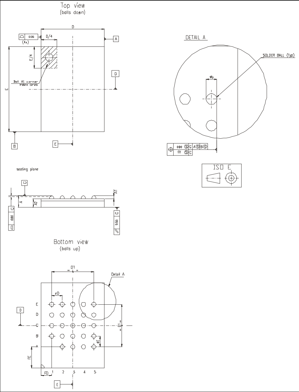
Figure 112. TBGA - 6 x 8 mm, 24-ball, mechanical package outline
