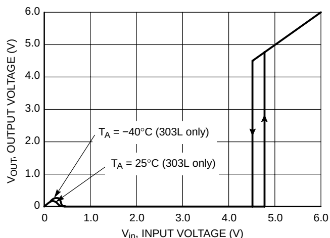
Figure 11. NCP302L/3L Series 4.5 V Reset Output Voltage vs. Input Voltage
