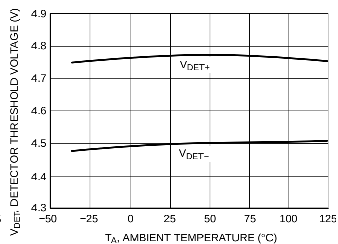
Figure 8. NCP302/3 Series 4.5 V Detector Threshold Voltage vs. Temperature
