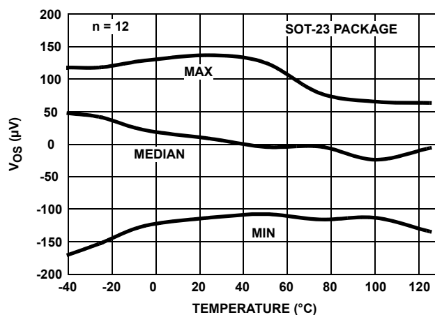
FIGURE 36. INPUT OFFSET VOLTAGE vs TEMPERATURE V_S = \pm 1.2V
