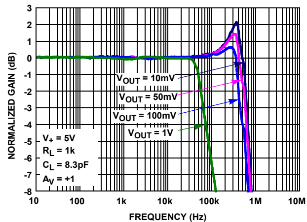
FIGURE 4. GAIN vs FREQUENCY vs V_{OUT} , R_L = 1k
