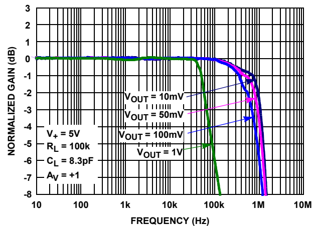
FIGURE 6. GAIN vs FREQUENCY vs V_{OUT} , R_L = 100k
