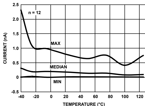
FIGURE 32. INPUT OFFSET CURRENT vs TEMPERATURE V_S = \pm 1.2V
