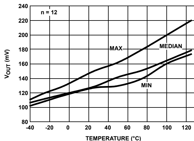
FIGURE 40. NEGATIVE V_{OUT} vs TEMPERATURE R_L = 1k V_S = \pm 2.5V
