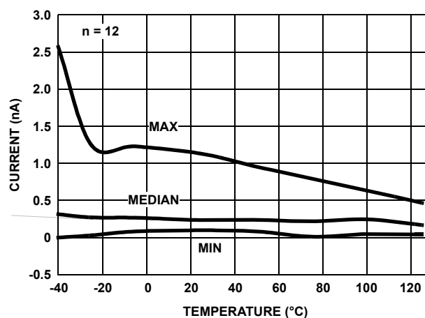
FIGURE 28. I_{\text{BIAS}} (+) vs TEMPERATURE V_S = \pm 1.2V
