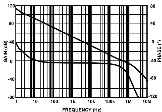
FIGURE 2. A_{VOL} vs FREQUENCY AT 100k \Omega LOAD
