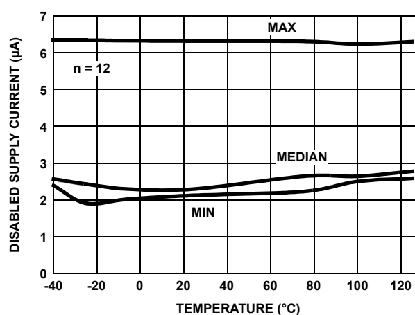
FIGURE 26. DISABLED SUPPLY CURRENT vs TEMPERATURE V_S = \pm 2.5V R_L = \text{INF}
