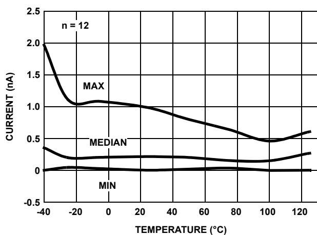
FIGURE 27. I_{\text{BIAS}} (+) vs TEMPERATURE V_S = \pm 2.5V
