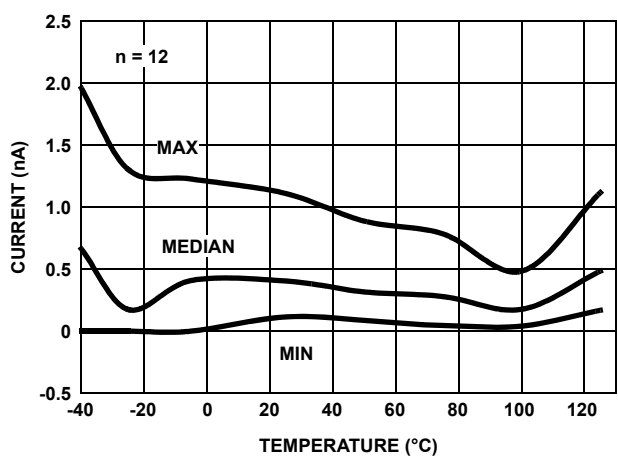
FIGURE 29. I_{\text{BIAS}} (-) vs TEMPERATURE V_S = \pm 2.5V
