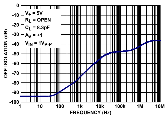
FIGURE 14. OFF ISOLATION vs FREQUENCY; V_+ , V_- = \pm 2.5V
