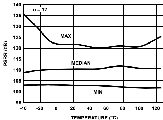
FIGURE 38. PSRR vs TEMPERATURE V_S = \pm 1.2V TO \pm 2.5V
