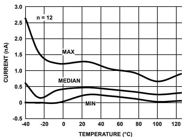
FIGURE 30. I_{\text{BIAS}} (-) vs TEMPERATURE V_S = \pm 1.2V
