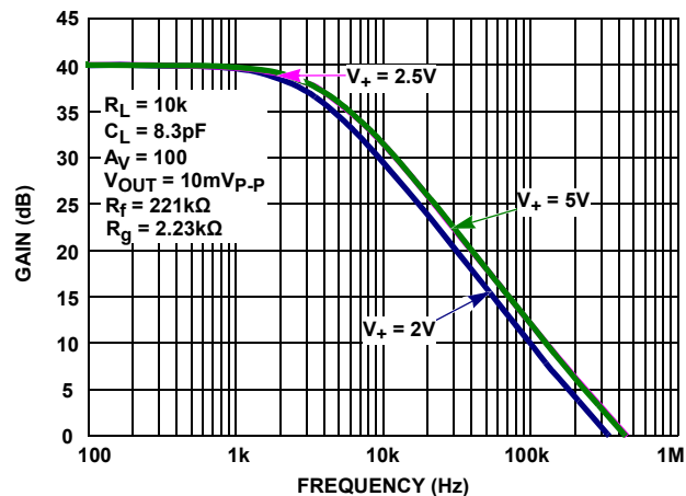
FIGURE 10. GAIN vs FREQUENCY vs SUPPLY VOLTAGE
