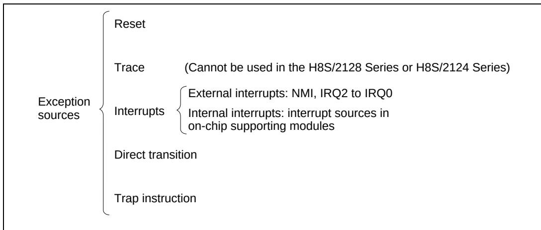
Figure 4.1 Exception Sources
