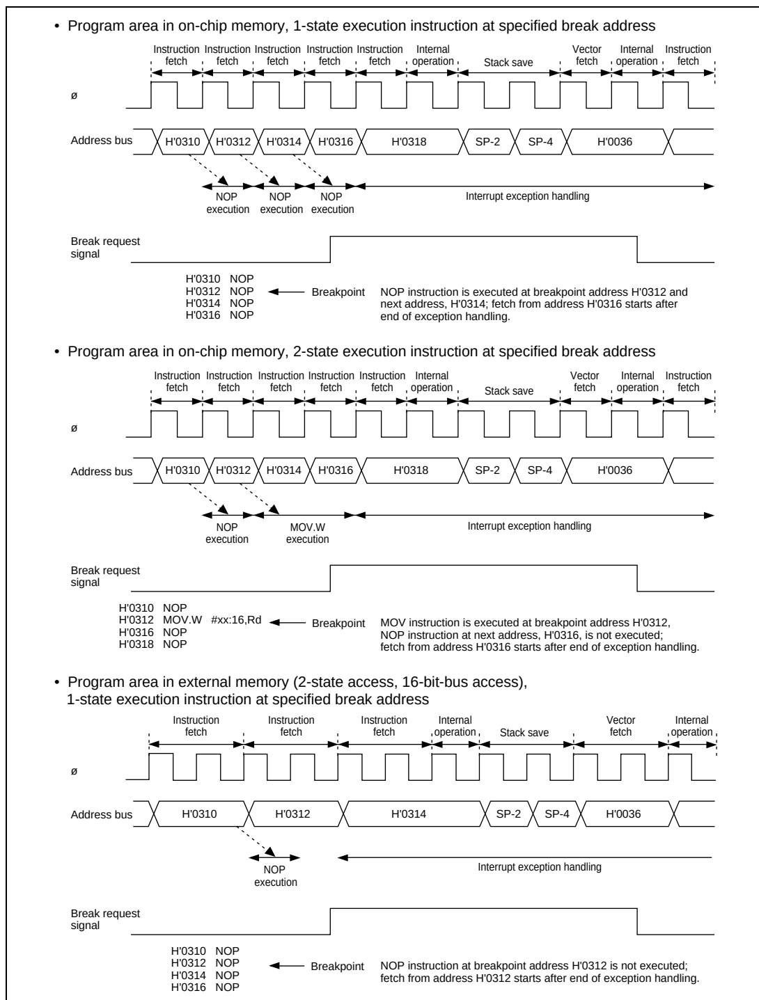
Figure 5.5 Examples of Address Break Timing
