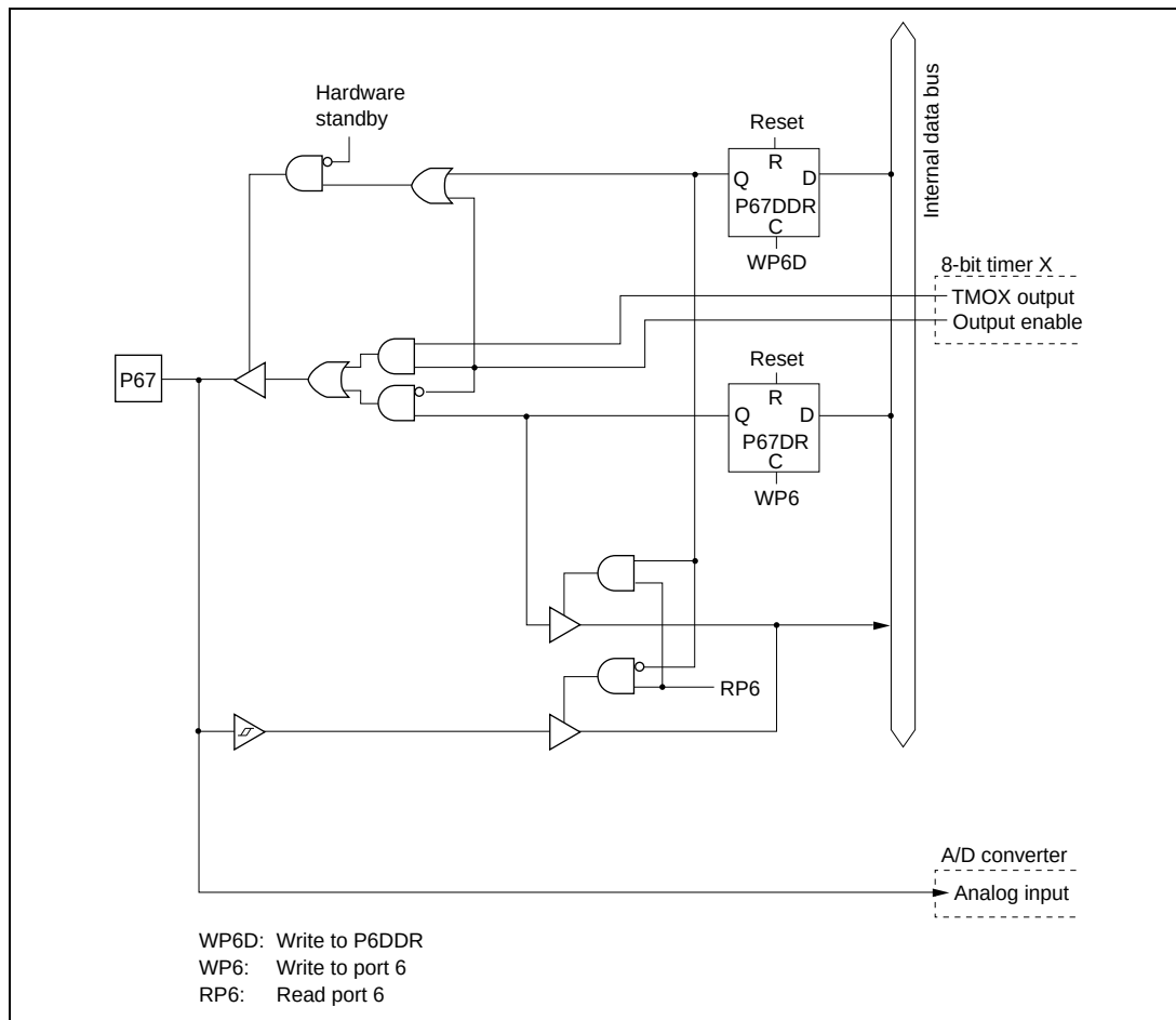
Figure C.22 Port 6 Block Diagram (Pin P67)
