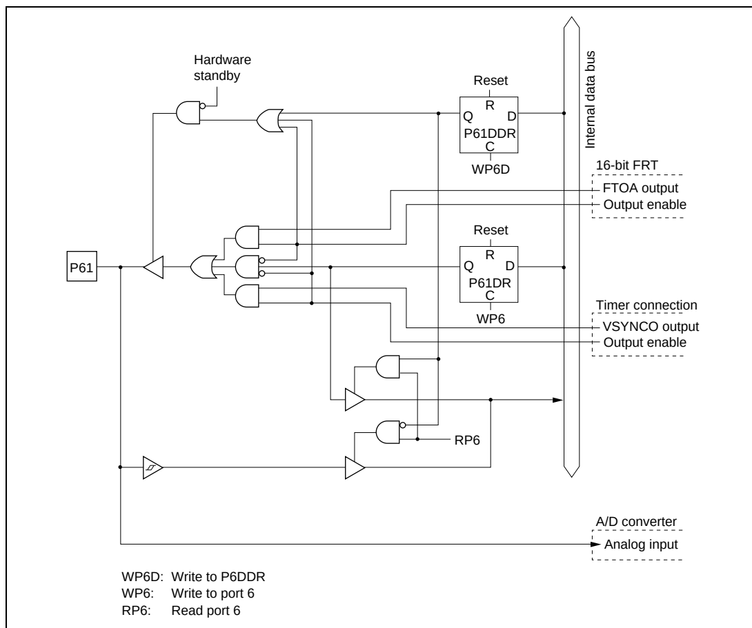
Figure C.19 Port 6 Block Diagram (Pin P61)
