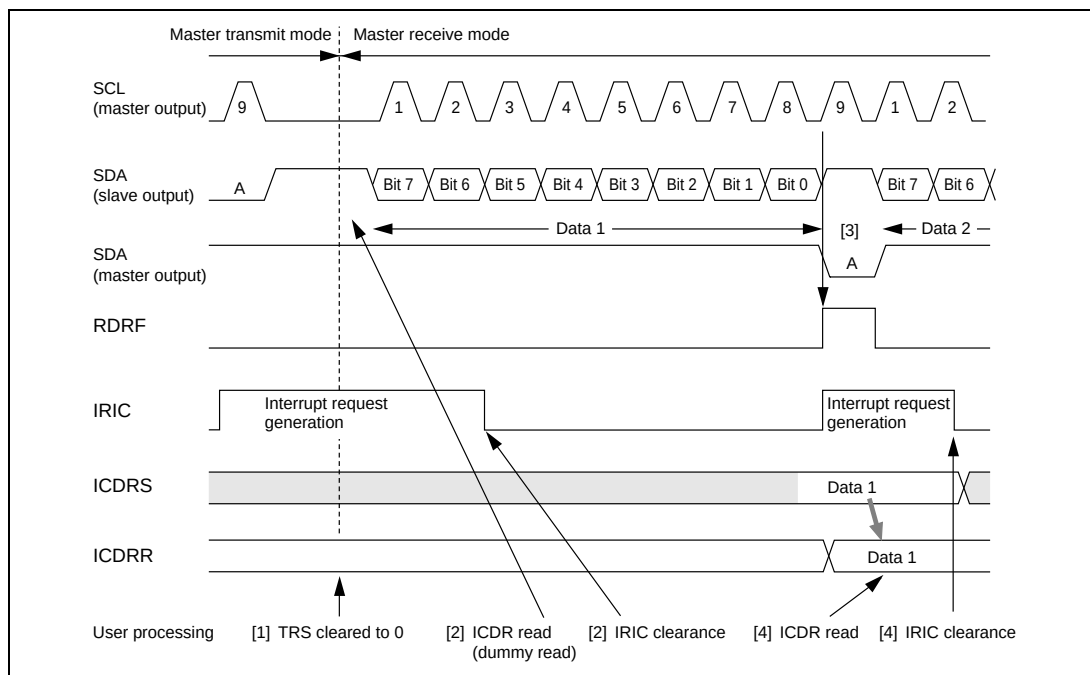
Figure 16.8 Example of Master Receive Mode Operation Timing (MLS = WAIT = ACKB = 0)
