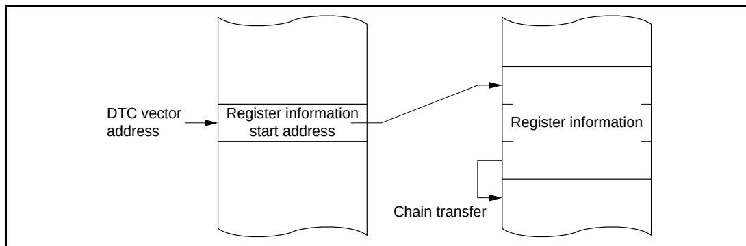
Figure 7.4 Correspondence between DTC Vector Address and Register Information
