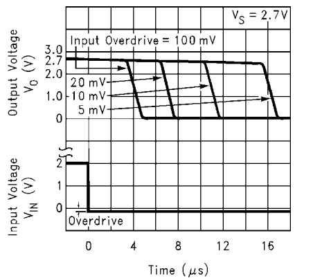
Response Time for Various Input Overdrives -t_{PHL}
