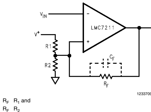
FIGURE 4. Positive Feedback for Hysteresis
