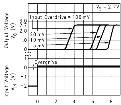
Response Time for Various Input Overdrives -t_{PLH}
