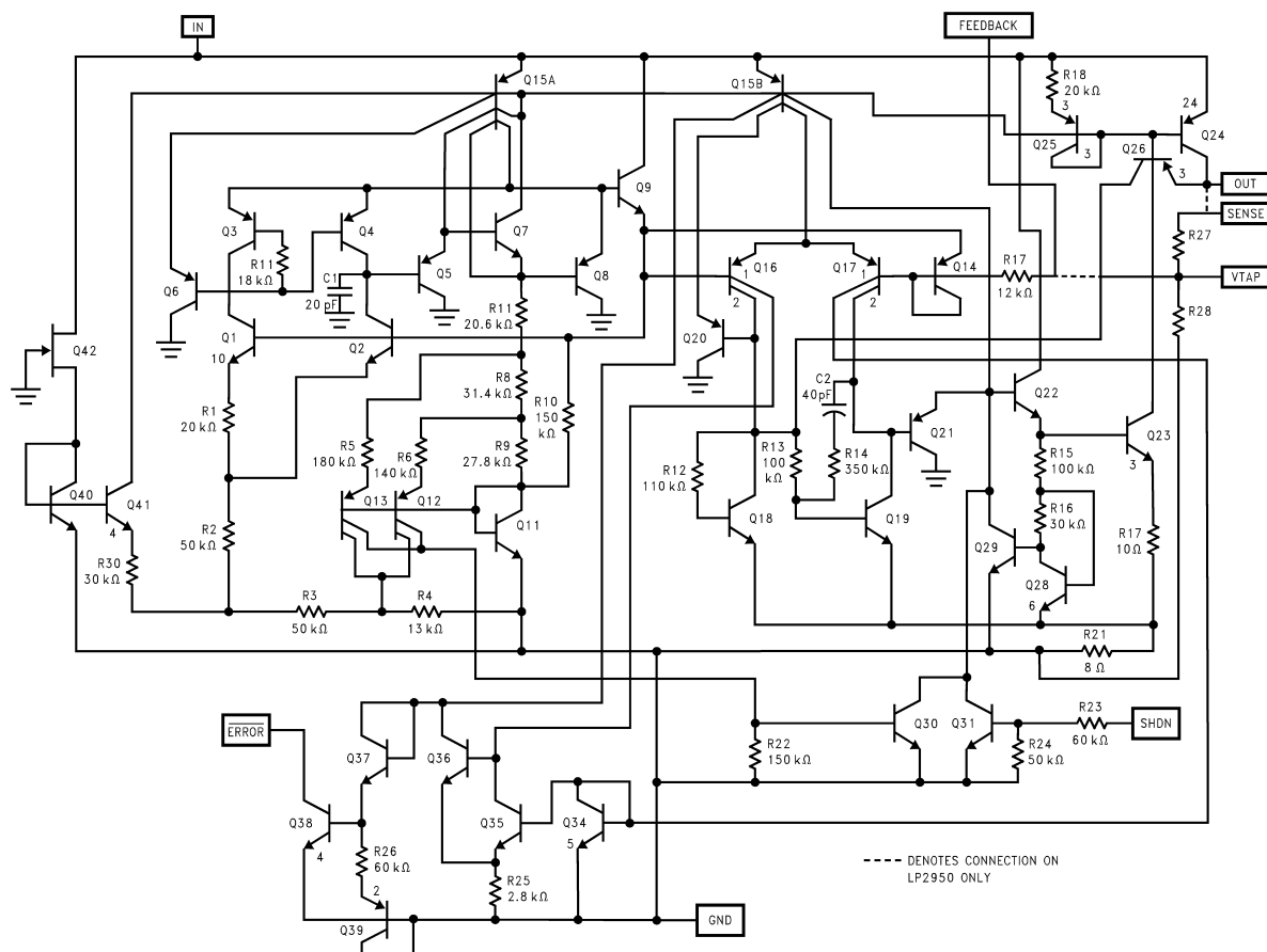
Figure 35. Schematic Diagram
