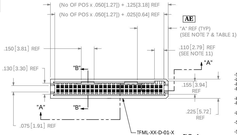
FIG. 1 -01: THROUGH HOLE
