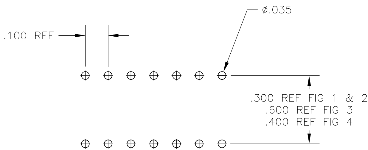
P.C.B HOLE LAYOUT TOLERANCE ±.003
