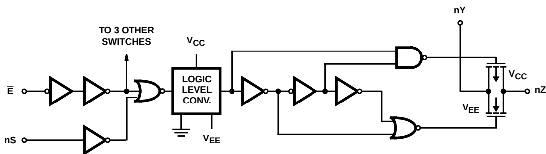
FIGURE 1. ONE SWITCH
