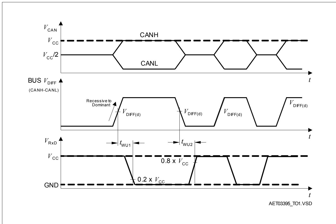
Figure 6 Wake-up behavior
