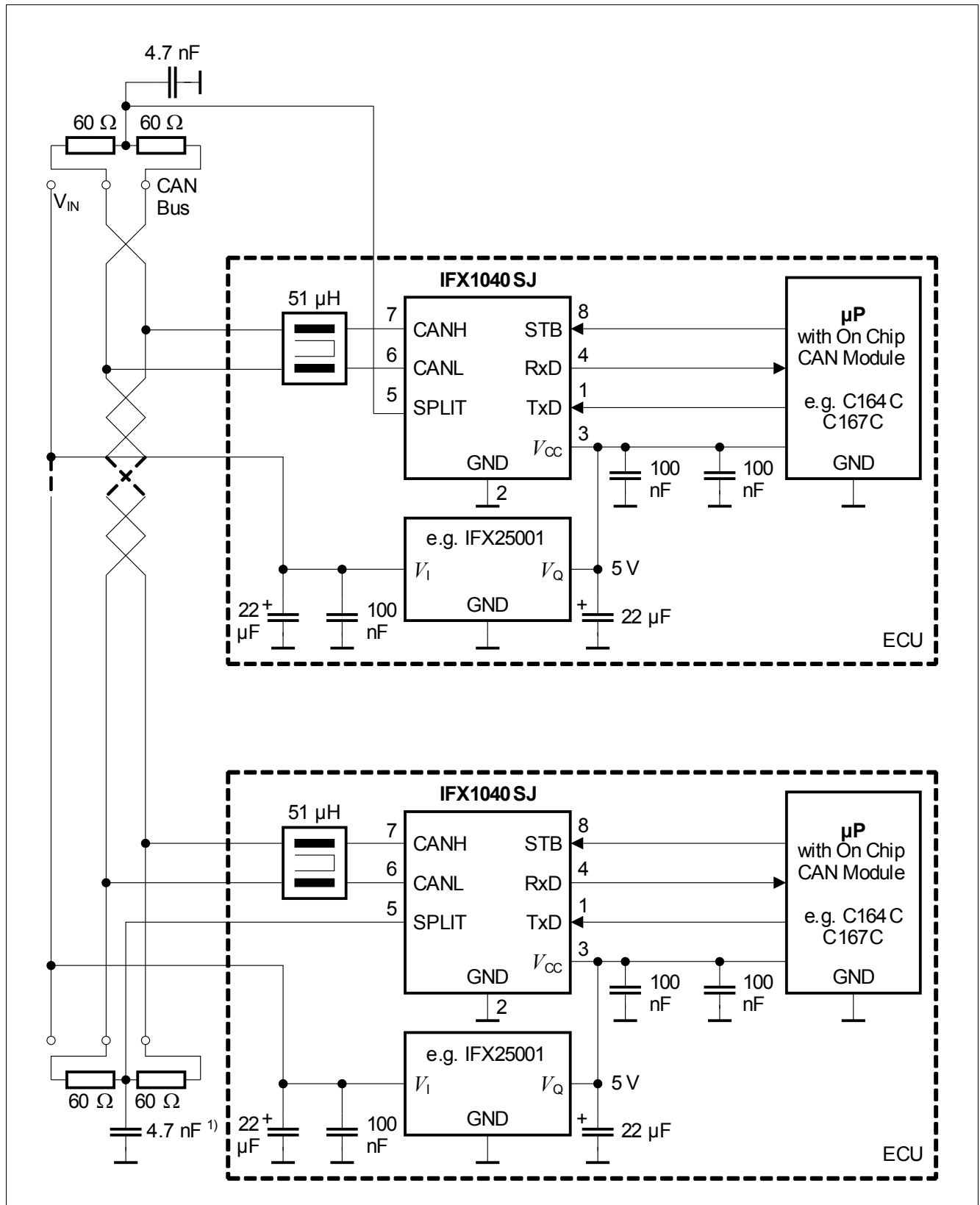
Figure 10 Application Circuit
