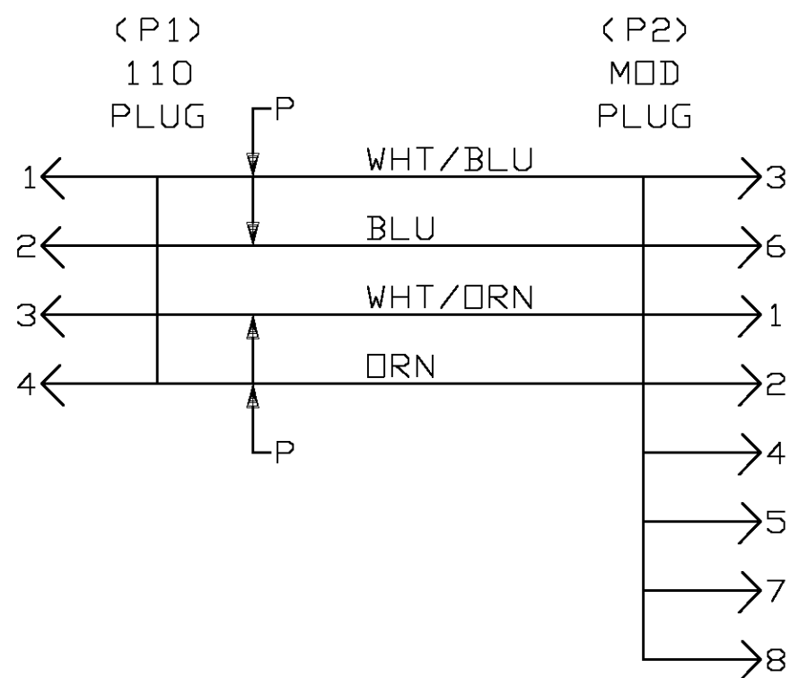
WIRING DIAGRAM 10/100 BASE-T
