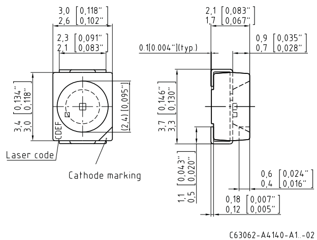
Figure 24: TOPLED
