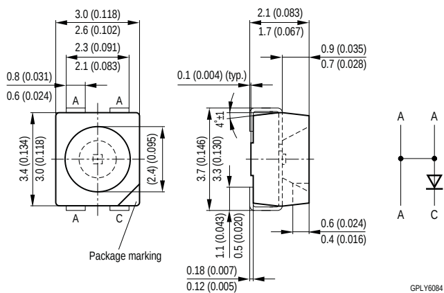
Figure 11: Power TOPLED
