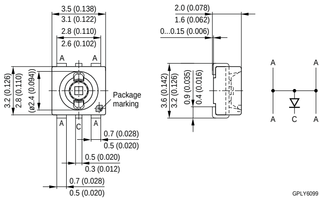
Figure 11: Power TOPLED
