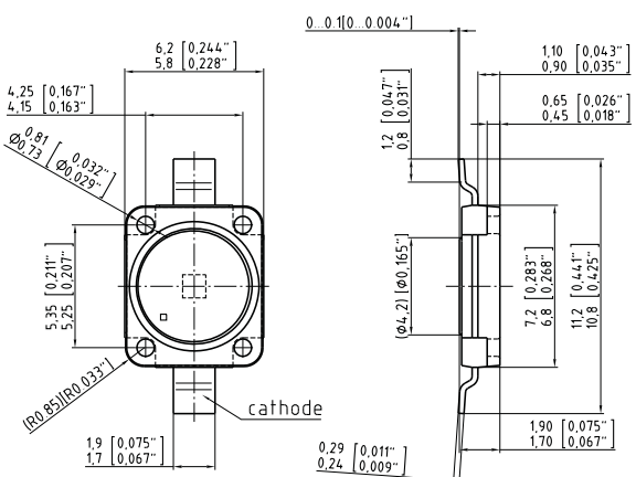
Figure 6: Golden DRAGON
