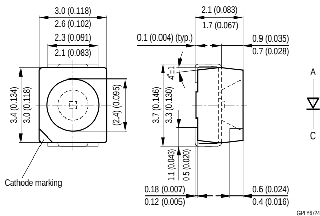
Figure 23: Mini TOPLED
