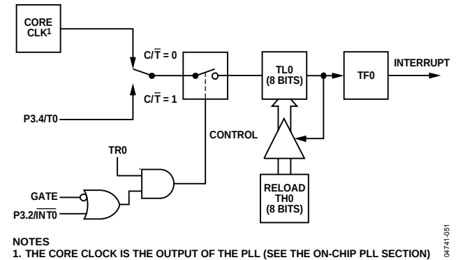
Figure 54. Timer/Counter 0, Mode 2
