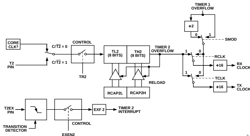
Figure 60. Timer 2, UART Baud Rates
