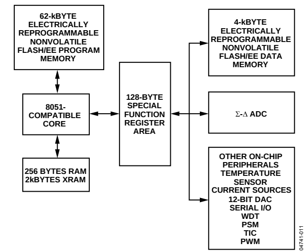
Figure 11. Programming Model
