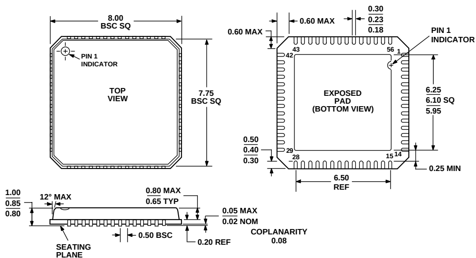
Figure 82. 56-Lead Lead Frame Chip Scale Package [LFCSP]
