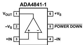
Figure 3. 6-Lead SOT-23 (RJ)
