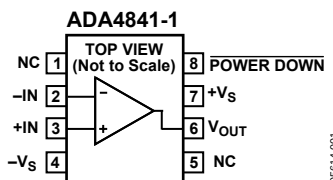
Figure 1. 8-Lead SOIC (R)
