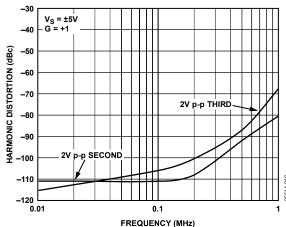
Figure 4. Harmonic Distortion
