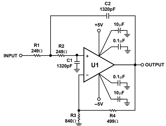
Figure 50. Two-Pole 500 kHz Reconstruction Filter Schematic
