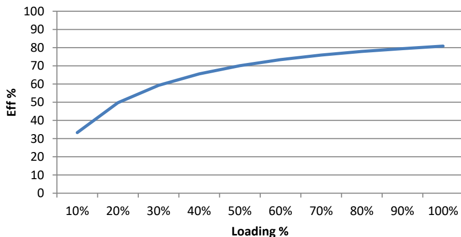
AM1L-2424S-NZ Efficiency vs. Loading
