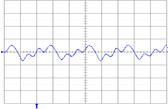
Fig. 1.8V.7: Output voltage ripple (20 mV/div.) at full rated load current into a resistive load with C_o = 10 \mu\text{F} tantalum + 1\mu\text{F} ceramic and V_{in} = 48 \text{ V} . Time scale: 1 \mu\text{s}/\text{div} .
